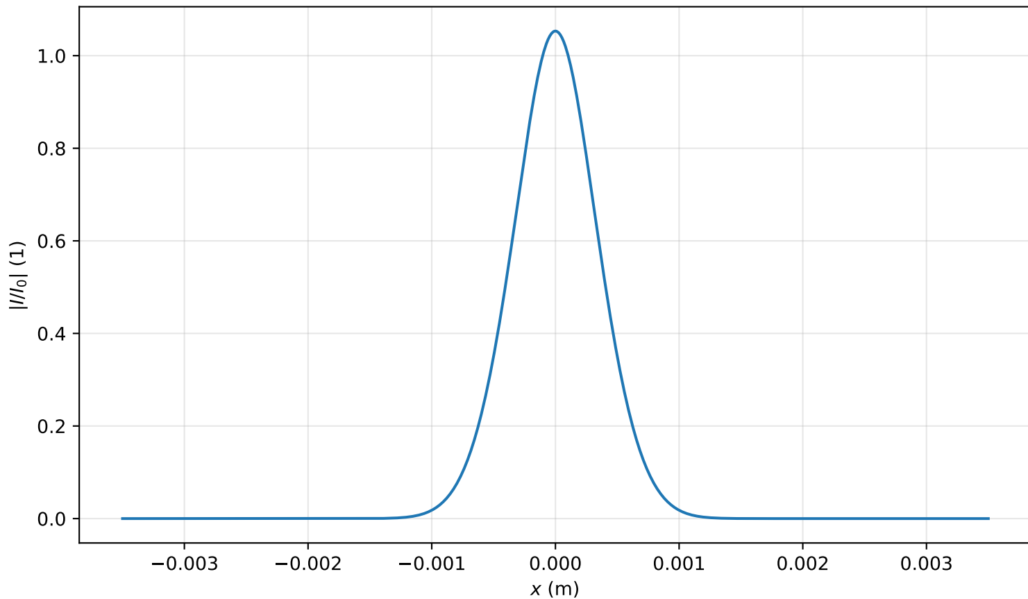
Intensity profile I(x, y = 0, z = 0.318m)/I_0 , P_{in}=0.8P_{cr} , artificial time
